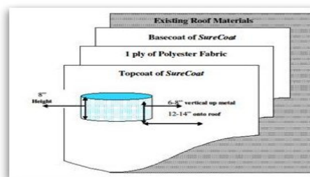
The SureCoat Roof System Design showing the layers of a SureCoat 3-ply Roof System
